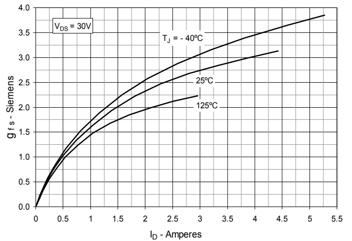
Fig. 10. Transconductance
